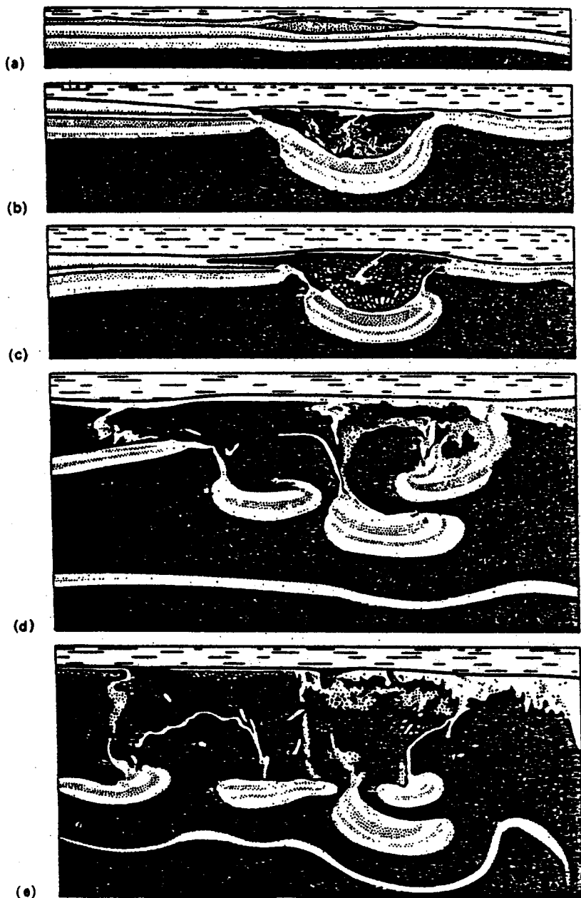
Fig. 5-27 Formation of pseudonodules in an experiment by Kuenen (1958). A layer of sand, locally thickened (a) and overlying unconsolidated clay, was vibrated. Load structures developed (b and c) and became completely enclosed in clay (d and e).
