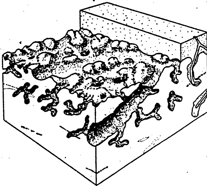
Figure 16. Sharply outlined burrows produced by excavating shrimp. Note the branching morphology of the burrows, which are up to 2 inches in diameter and can extend 6 feet or more below the bedding plane surface at which they originate.
