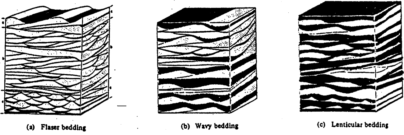
Figure 7. Gradations in flaser bedding, from flaser to wavy to lenticular, with increasing mud content.
