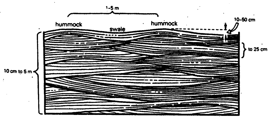
Figure 1.26 Hummocky cross stratification.
