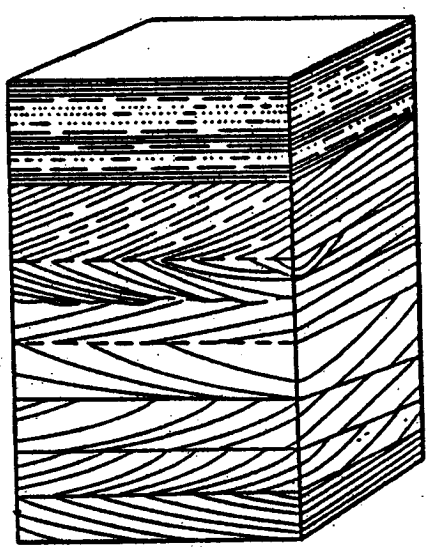
Figure 8. Herringbone cross-stratification. Note cross-beds dipping in opposite directions.
