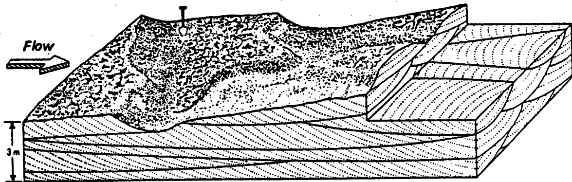
Figure 6. Trough cross-stratification.
