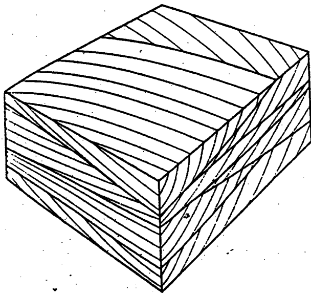
Figure 5. Wedge cross-stratification.
