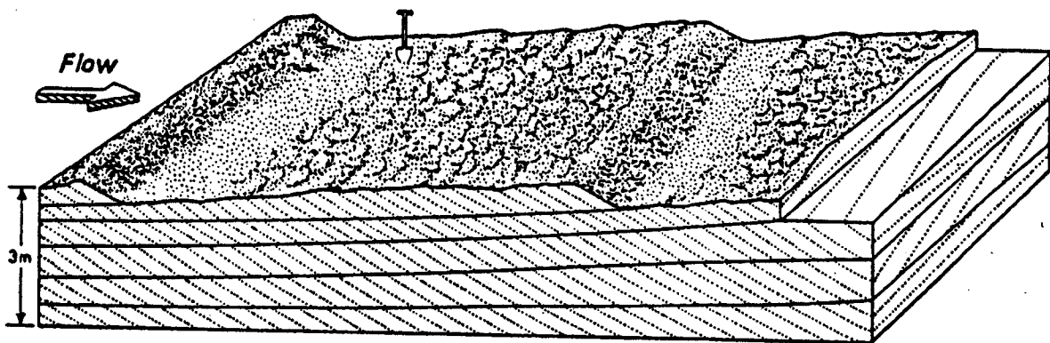
Figure 4. Tabular cross-stratification.
