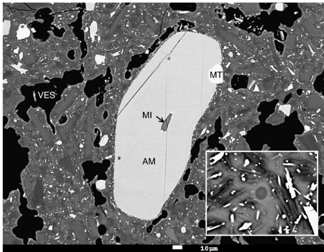
Fig. 7. Backscattered electron image of andesite from 4 November, 2010. Sample is from a prismatically jointed juvenile block collected from a pyroclastic flow deposit in Kali Gendol. The large grain at the center of the image is a nearly euhedral amphibole (AM) phenocryst which has a very thin (or absent) reaction rim and a melt inclusion (MI) with 1200ppm S. The bright white grains in the image are magnetite (MT), black areas are vesicles (VES), and the groundmass contains abundant plagioclase, pyroxene and magnetite microlites and interstitial glass. Other areas of the sample contain abundant complexly zoned plagioclase, clinopyroxene and orthopyroxene. The inset enlargement shows detail of the groundmass: elongate dark microlites are plagioclase, bright grains are magnetite and pyroxene and the intermediate gray areas are 66–68% SiO 2 glass. The circular spot is a 5 μm-diameter electron beam damage area.
