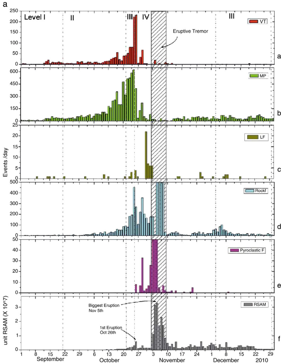
Fig. 3. (a) Daily count of the seismicity recorded at Merapi during 2010 eruption. VT = Volcano-tectonic; MP = Multiphase (=Hybrid earthquake); LF = low-frequency; Rockf = Rockfall earthquakes; Pyroclastic F = Pyroclastic flows; RSAM = Real-time Seismic Amplitude Measurement. (b) Location of VT earthquakes prior and during the eruption.
