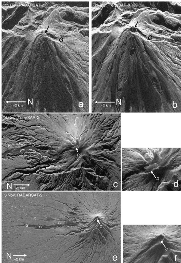
Fig. 4. Synthetic Aperture Radar (SAR) images of the summit of Merapi volcano before and after the times of the 26 October explosive eruption and the 4 November explosive eruptions. For clarity, images are oriented with respect to line of sight of the radar. Arrows indicate north (N) direction and approximate scale. G (Kali Gendol), K (Kali Kuning), KJ (Kinahrejo). a, RADARSAT image, 11 October, 2009. Arrow indicates the 2006 lava dome. b, TerraSAR-X image, 26 October, showing new summit crater (arrow) produced by explosive eruption of 26 October. c, TerraSAR-X image, 4 Nov 2010, showing large ( \sim 5 \times 10^6 \text{ m}^3 ) lava dome (D). Pyroclastic flow deposits (PF) from the 26 October eruption appear dark in the radar images. d, Enlargement of the summit area of image a. e, RADARSAT image of 5 November, 2010, showing pyroclastic flow deposits (PF, dark gray) and surge deposits (S, light gray). These deposits formed earlier during the main phase of the 4–5 November explosive eruption. An enlarged, elongate crater, produced by the November 4–5 eruption is also evident at the summit. f, Enlargement of the summit area of image c.
