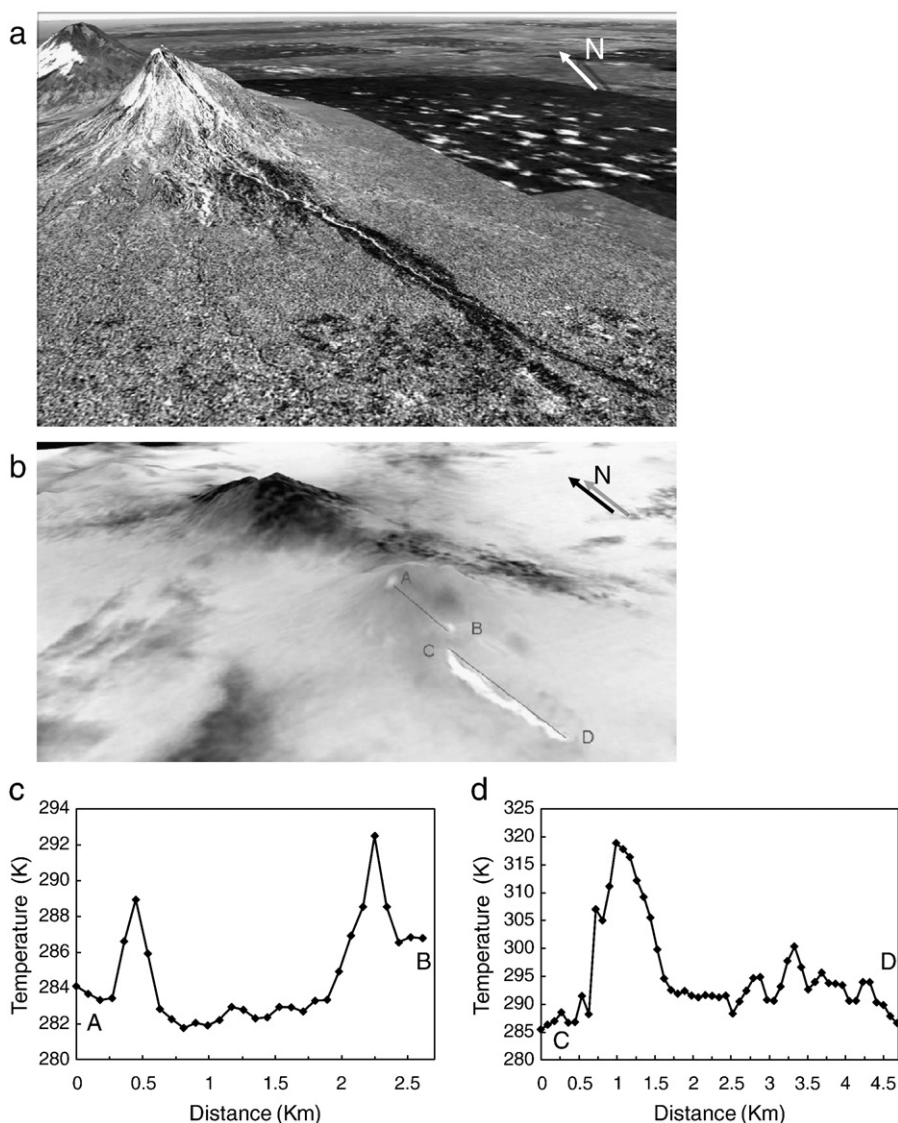
Fig. 6. Pyroclastic flow deposits illustrated using SAR change detection and thermal channel of ASTER data. a, Perspective view of SAR change detection analysis performed using two COSMO-SkyMed data acquired on 1 May 2010 and 11 November 2010; the image shows the deposits (black areas) around the pre-eruption channel (white pixels inside black areas). A total length of about ~15 km and a covered area of 13 km 2 have been estimated from this analysis. b, Perspective view of temperature image from ASTER data acquired over Merapi (foreground) and Merbabu (background) volcanoes on 1 November 2010 (night time); elevated temperatures signify the deposit of the pyroclastic flow of 26 October. The two temperature profiles along the pyroclastic flow show retrieved temperatures integrated across the 90×90 m 2 sensor footprint, total length of the hot area detected by ASTER is ~7.2 km (A–B plus C–D segments), corresponding to the portion of the 26 October flow deposit still very hot on 1 November.
