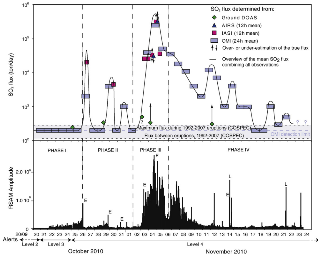
Fig. 9. Comparison between SO 2 fluxes and RSAM data. top, Overview of SO 2 degassing during the 2010 Merapi volcano eruption (UTC time). SO 2 fluxes were determined from ground-based scanning DOAS measurements (mean fluxes measured over hour-long intervals) and satellite images, from IR IASI and AIRS sensors (mean fluxes calculated for 12h intervals) and the UV OMI sensor (mean fluxes calculated for 24h intervals). OMI is more sensitive than IR sensors to lower tropospheric plumes (<5 km altitude). Therefore, when the plume is weaker, OMI was the primary source of mean SO 2 flux estimates. The black line has been manually added to interpolate between discrete values of the SO 2 flux to highlight degassing trends. Ranges for SO 2 emissions during and between eruptions taking place between 1999 and 2007 are from scanning correlation spectrometer (COSPEC) measurements (Nho et al., 1996; Humaida et al., 2007). Question marks indicate gaps in OMI data coverage, or interference from SO 2 plumes emitted by other Indonesian volcanoes. Refer to the text for explanations concerning the reasons of over or under-estimations of the true flux. bottom, RSAM computed for the Plawangan station (6 km from the summit). A clear correspondence between RSAM and SO 2 flux is demonstrated, supporting our identification of four distinct phases to the eruption (indicated by Phases I to IV). E stands for explosion; L for Lahar.
