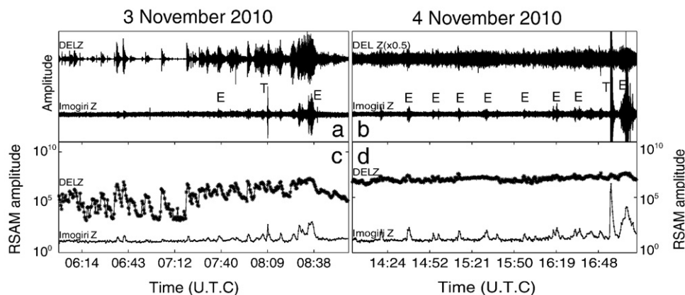
Fig. 5. Record of the seismic amplitude at Imogiri station located 46 km south of Merapi volcano. a, Normalized vertical component signals recorded at a proximal station (DEL, Deles, 4 km from Merapi's summit) and at a distal station (CRM, Imogiri, 46 km south) during the 3 November explosion sequence. T symbols indicate small ( M < -1 ) tectonic earthquakes on the Opak fault, E symbols indicate explosions at the Merapi volcano summit. b, Same as a for data from 4 November. c, RSAM computed for stations DEL and CRM (Imogiri) on 3 November. Note that RSAM at DEL is multiplied by 10^8 for clarity. d, Same as c for data from 4 November.
