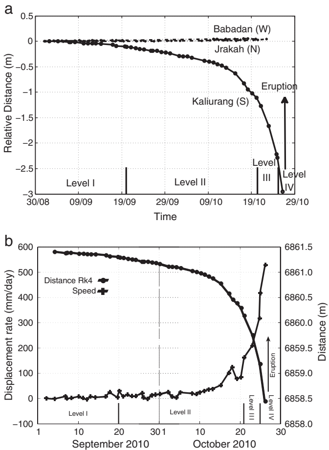
Fig. 2. Electronic Distance Measurement data for lines between observatory posts and the summit of Merapi (see Fig. 1). Reflectors near the summit of the volcano were destroyed by the eruption of 26 October, preventing further observations. Shortening of EDM lines between the volcano’s summit and flanks is indicative of pressurization and inflation of the upper part of the volcano with magma, whereas increasing distances indicates deflation. (a) EDM observations for 3 lines Babadan-summit (West) Jrahkah-summit (North) and Kaliurang-summit (Rk4 reflector, South). “Relative Distance” refers to the change in line length with respect to time, reference taken arbitrarily on 1 September 2010. (b) Detail of the Kaliurang-summit EDM line, and displacement rate.
