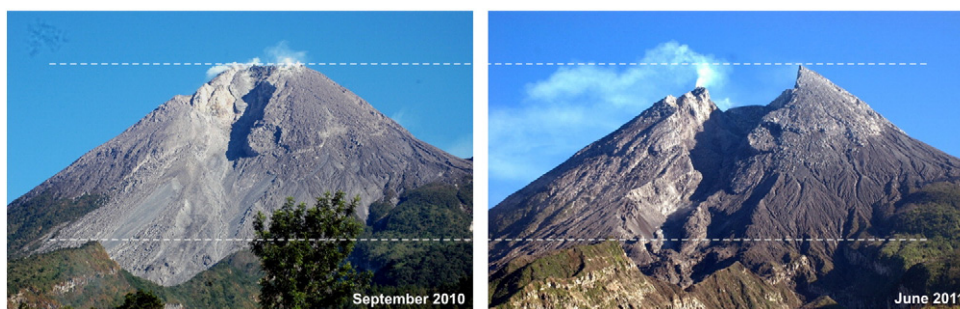
Fig. 10. Morphology of the summit area. a, Before the October–November eruption. b, After the eruption. Depth of the new crater is about 200 m.
