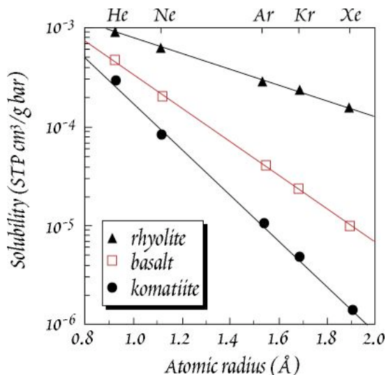
Figure 7.4. Solubility of the rare gases in melts of varying composition at 1200^\circ to 1400^\circ C. Solubility is a strong function of atomic radius and melt composition, but only a weak function of temperature. From Carroll and Draper (1994).
