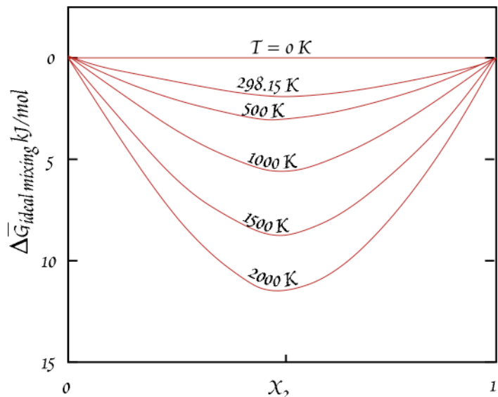
Figure 3.6. Free energy of mixing as a function of temperature in the ideal case.
