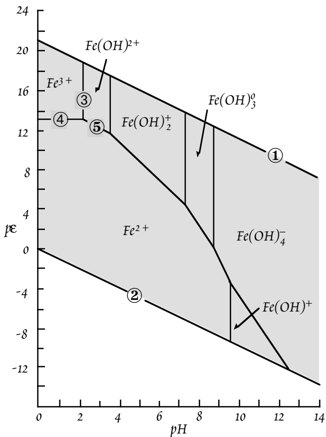
Figure 3.19. pε—pH diagram showing predominance regions for ferric and ferrous iron and their hydrolysis products in aqueous solution at 25°C and 1 bar.
