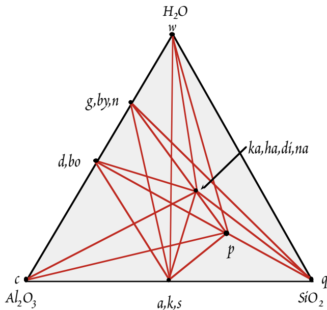
Figure 3.2. Phase diagram for the system Al 2 O 3 -H 2 O-SiO 2 . The lines are called joins because they join phases. In addition to the end-members, or components, phases represented are g: gibbsite, by: bayerite, n: norstrandite (all polymorphs of Al(OH) 3 ), d: diaspore, bo: boehmite (polymorphs of AlO(OH)), a: andalusite, k: kyanite, s: sillimanite (all polymorphs of Al 2 SiO 5 ), ka: kaolinite, ha: halloysite, di: dickite, na: nacrite (all polymorphs of Al 2 Si 2 O 5 (OH) 4 ), and p: pyrophyllite (Al 2 Si 4 O 10 (OH) 2 ). There are also 6 polymorphs of quartz (coesite, stishovite, tridymite, cristobalite, α-quartz, and β-quartz).
